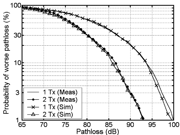
Figure 7. Path loss probability distribution within the measured and simulated building.
