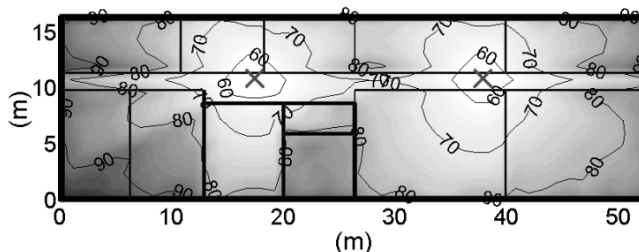
Figure 10, Simulated path loss for two transmitters. The X shows the location of the transmitters.
