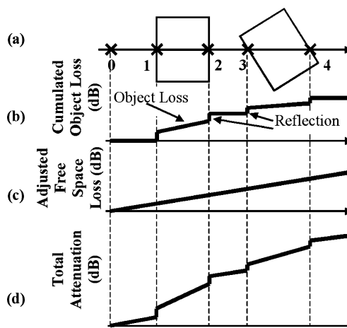
Fig. 8. Attenuation calculations for a ray passing through two objects.
