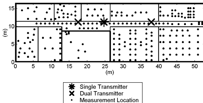
Fig. 3. Path-loss measurement locations in the ECE building. Lines represent internal walls. The thin lines are plaster board walls, and the thick ones are concrete walls.
