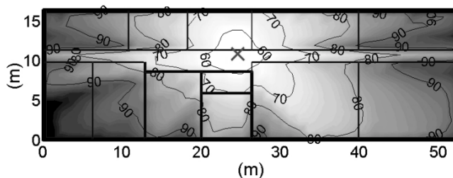
Figure 9, Simulated path loss for one transmitter at 990 MHz. The X shows the transmitter location.
