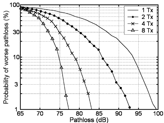
Figure 11, Cumulative probability distribution for simulated results, showing the result for one, two, four and eight transmitters.
