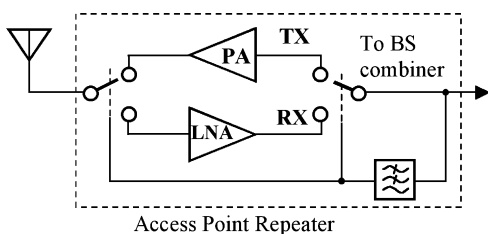
Fig. 2. Possible implementation of an APR.
