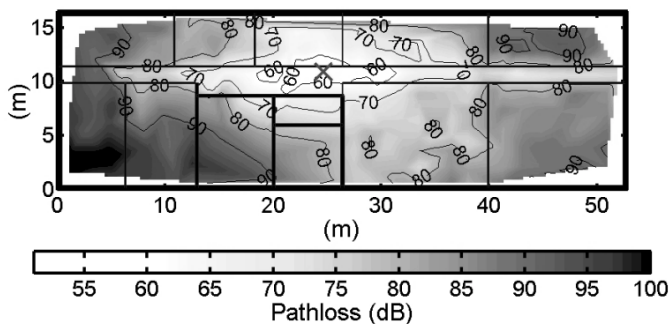
Fig. 5. Measured path loss with one transmitter over the area of the building at 990 MHz. The dark lines are the internal walls. The X shows the location of the transmitters.
