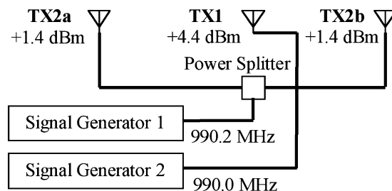
Fig. 4. Transmitter set up simulating Access Point Repeaters. The total transmitter power from T x2a and Tx2b were matched to the Tx1 power.
